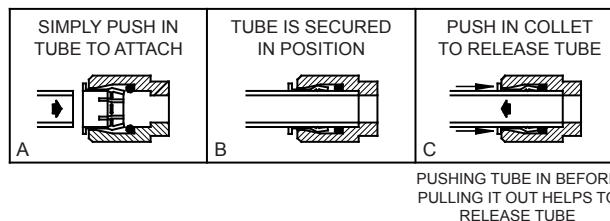
Figure 13 – Quick Connect Fittings
